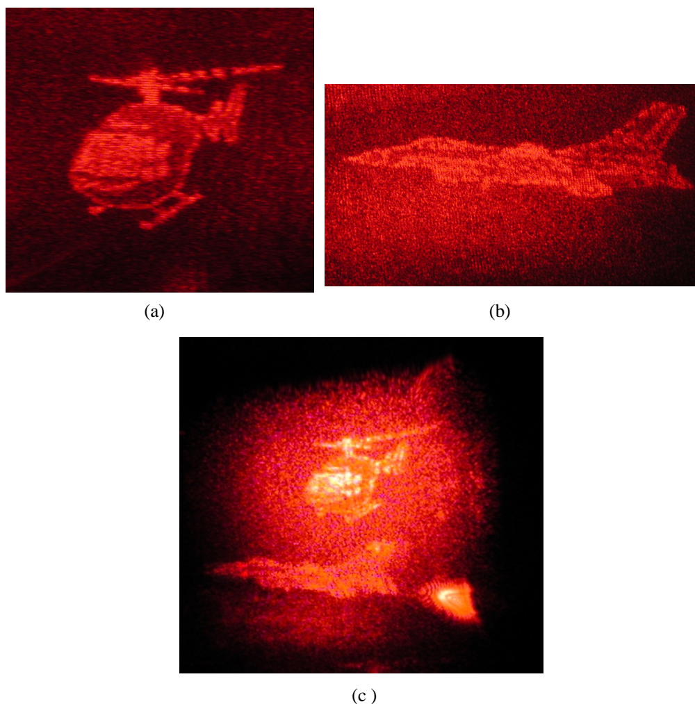
Fig. 4. (a) The reconstructed portion of the real 3-D image at 30 cm from the converging lens, (b) the reconstructed portion of the real 3-D image at 27.5 cm from converging lens, and (c) the virtual image looking into the DMD, the conventional way to view a hologram. The photographs were taken with a Nikon Coolpix990 digital camera.
