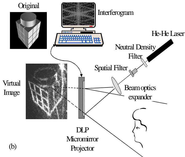
Fig. 1. Schematic of DMD hologram projection system for (a) real and (b) virtual images.
