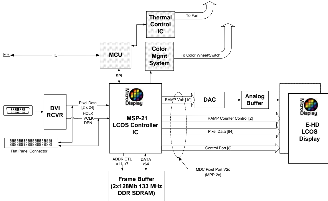
Typical system using the MD1920P4
