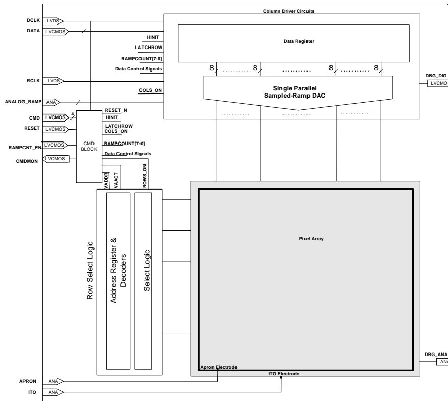
Internal architecture of the MD1920P4
