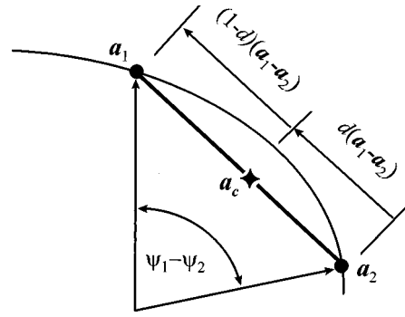
Fig. 1 Geometric relationships for pseudorandom encoding the desired value \mathbf{a}_c using random binary selection of modulator values \mathbf{a}_1 and \mathbf{a}_2 .
