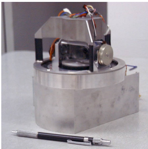
Figure 1: Two-Axis Scanning Laser Rangefinder. (a) Prototype (b) CAD cross-section
