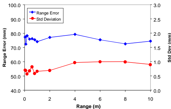
Figure 2: Range error and deviation vs. distance
