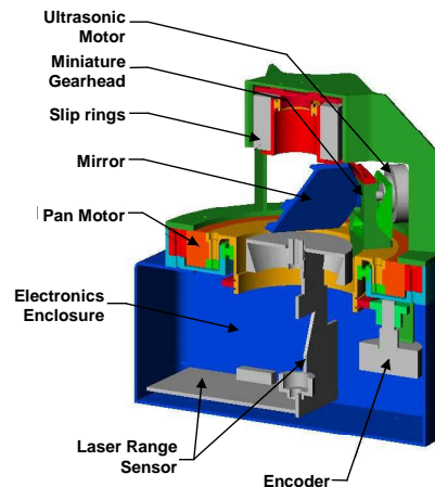
Figure 1: Two-Axis Scanning Laser Rangefinder. (a) Prototype (b) CAD cross-section
