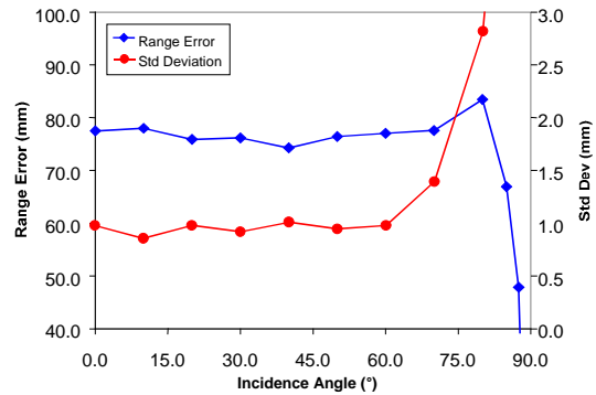
Figure 3: Range error and deviation vs incidence angle
